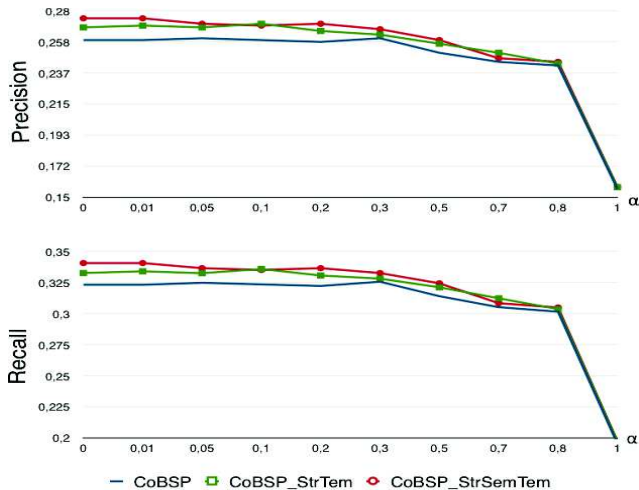
Fig. 2. Comparison of the precision (top) and the recall (bottom) of calculated social dimension of the COBSP algorithm (Blue), CoBSP_StrTem algorithm (Green) and CoBSP_StrSemTem algorithm (Red)
