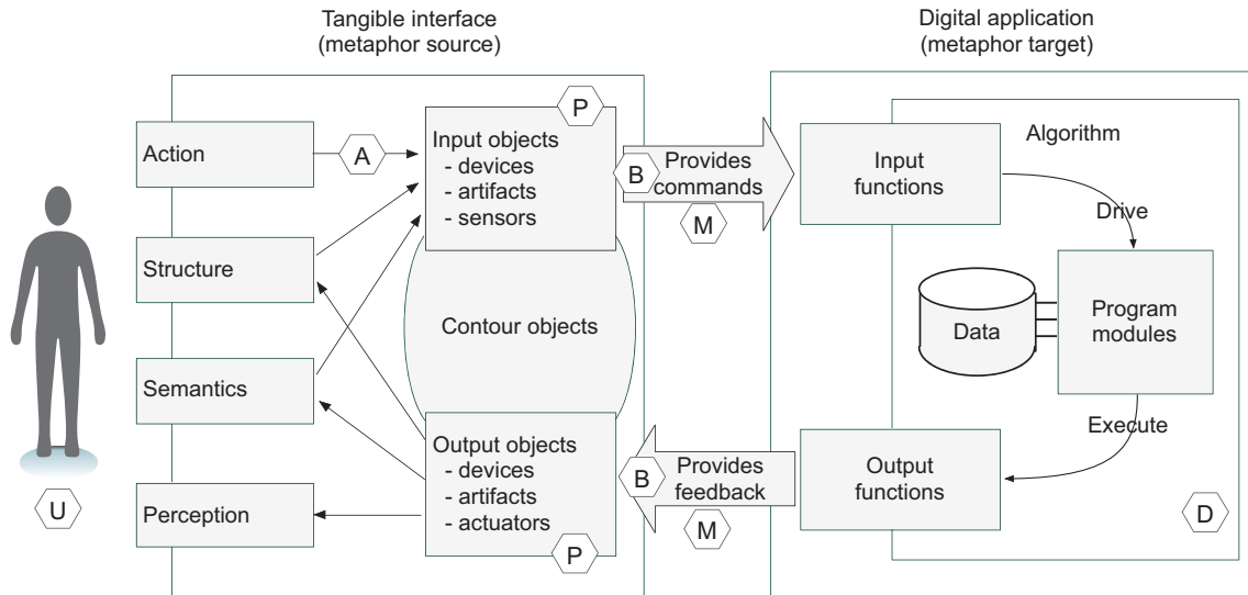
Fig. 4 Relations between metaphor and TUI components
