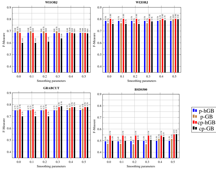
Figure 7: F_r -measure comparisons between the four segmentation results of p -hGB, p -GB, cp -hGB and cp -GB on each of the databases, BSDS500 , GRABCUT , WI1OBJ and WI2OBJ , under the ODS setting with the variation of the smoothing parameter \sigma from 0.0 to 0.5.
