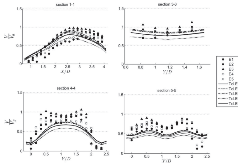
Fig. 6 Velocity magnitude in section 1-1, section 3-3, section 4-4 and section 5-5
