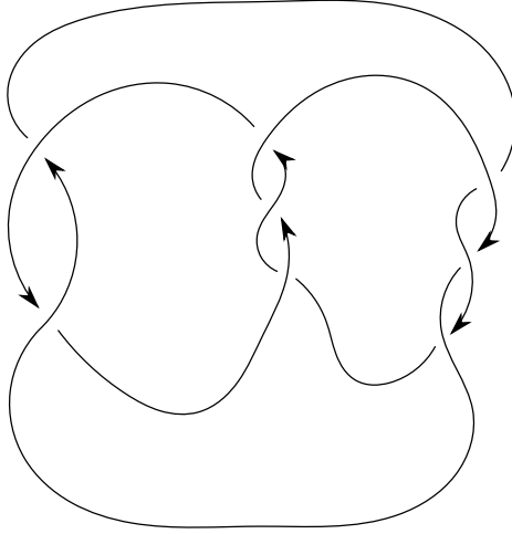
FIGURE 10. K(2, 3, -3) .
