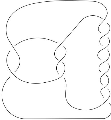
FIGURE 7. L(-2, 3, 7) .
