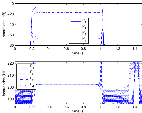
Figure 8: Simulation results. Transient on \gamma . Top: amplitudes of the first four partials of the mouthpiece pressure. Bottom: frequencies of the first four partials divided by their rank. \zeta = 0.6 , \gamma = 0.45 .
