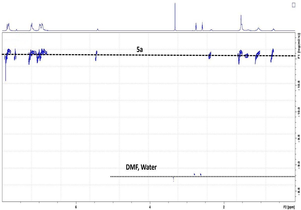
Figure 3. HR-DOSY spectrum of 5a in DMF, with the normal 1 H spectrum (top) and diffusion coefficients on the y-axis (side).
