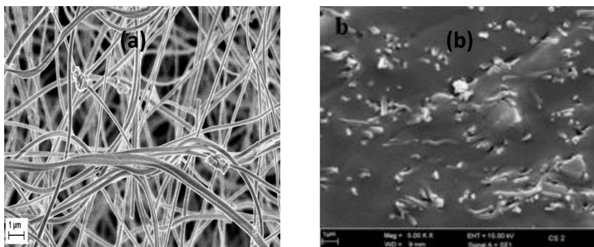
Figure 13: SEM micrographs of: (a). Palladium-silica ( \text{Pd-SiO}_2 ) nanofibres; (b). Nafion ® membrane comprising 3 wt% of \text{Pd-SiO}_2 nanofibres, adapted and reprinted with permission from reference 126, Copyright (2013) Elsevier.
