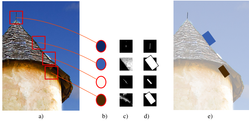
Fig. 1.3 The iterative approach of Shiraishi and Yamaguchi [20]. a) source image, b) pixel color for four sample pixels, c) difference between the pixel color and surrounding pixel colors is stored in an array, d) moment analysis of the array gives a rectangle with the same moments, e) for each anchor point, the attributes of the rectangle computed for this pixel are read to render the stroke.
