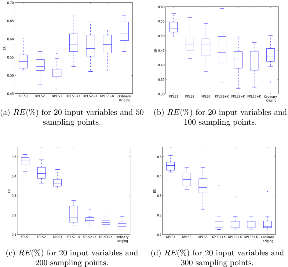
Figure 4: RE of the Griewank function in 20D over the interval [-5, 5] . The experiments are based on the 10-latin-hypercube design.
