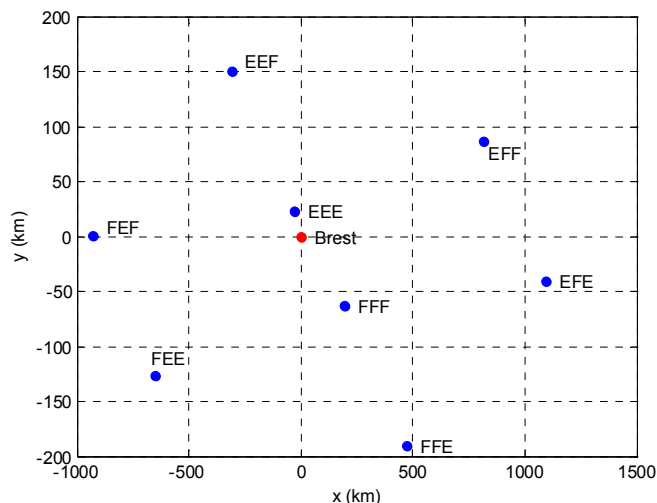
Fig. 7. Geolocation results using the ToA technique, as a function of the selected propagation modes.
