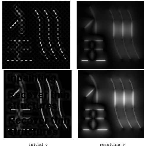
Fig. 7 Plots of the isotropy map M(v) \in \mathbb{R}^{\mathcal{P}} calculated from weights the v in RNLTV. The corresponding restored images u are in Figure 6. Top: for the checkerboard mask; Bottom: for the word mask. Left: initial guesses of the weights computed from the damaged image; Right: weights v after convergence of RNLTV.
