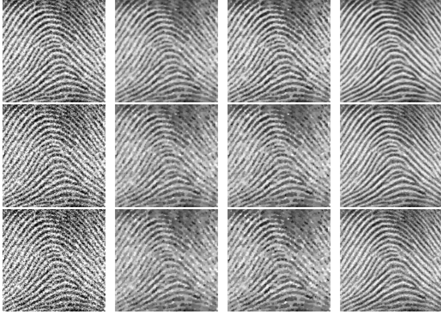
Fig. 17 Denoising results for the additive white Gaussian noise with standard deviation \sigma = 0.1, 0.16, 0.2 (from top to bottom).
