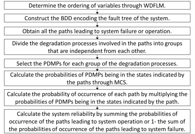
Fig. 6. The flowchart of the computational method.
