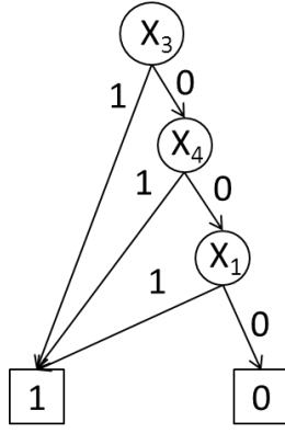
Fig. 5. BDD for fault tree in Fig. 3.
