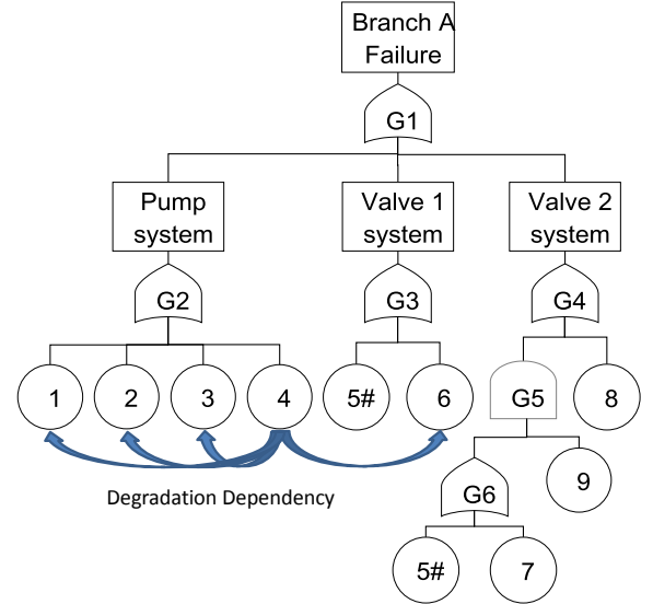
Fig. 8. The fault tree of one branch of the RHRS.
