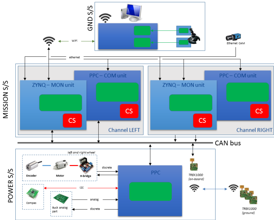
Figure 1: Architecture of the TwIRTeer
