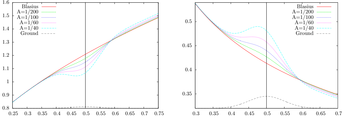
Figure 15 – Bump amplitude: displacement thickness \delta_1 (left) and zoom on the friction term \tau (right) – f_b(x) = A \exp(\frac{-(x-0.5)^2}{2(0.05)^2}) , T = 3 , J = 800 , \bar{\delta} = 10^{-3} , linear profile.
