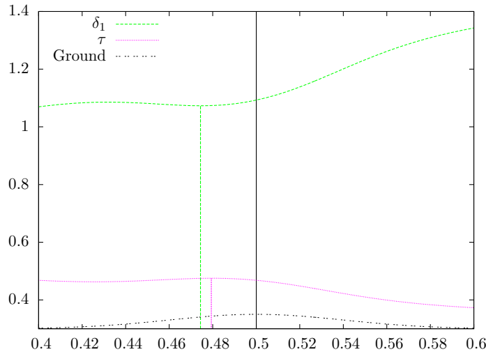
Figure 12 – Displacement thickness and friction term over a bump– f_b(x) = \frac{1}{50} \exp(-\frac{(x-0.5)^2}{2(0.04)^2}) , \bar{\delta} = 10^{-3} , T = 3 , J = 800 , linear profile. Maximum of friction term is in advance from the top of the bump.
