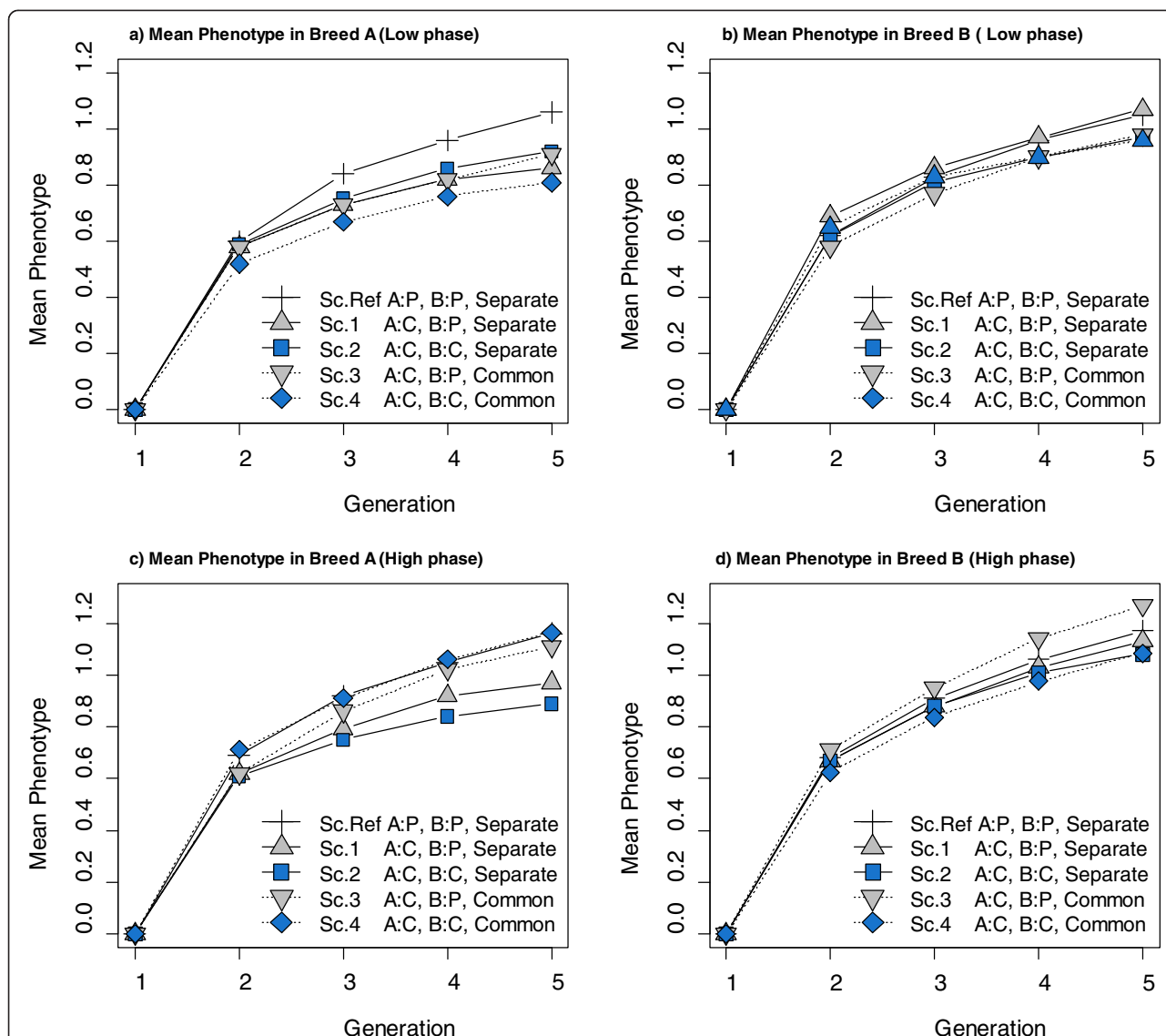
Figure 8 Mean phenotype of purebred individuals. (a) and (b) Results for a low correlation of LD phase between breeds A and B ( r=0.2 for markers 1 cM apart). (c) and (d) Results for a high correlation of LD phase between breeds A and B ( r=0.7 for markers 1 cM apart). The plotted responses are means from 30 replicates. Sc. Ref: Selection criteria in both breed A and B was for purebred performance (P) and both breeds had Separate training sets. Sc.1: Selection criteria in breed A was for crossbred performance (C) and selection criteria in breed B was for purebred performance and both breeds had separate training sets. Sc.2: Selection criteria in both breed A and B was for crossbred performance and both breeds had separate training sets. Sc.3: Selection criteria in breed A was for crossbred performance and selection criteria in breed B was for purebred performance and both breeds had a Common training set. Sc.4: Selection criteria in both breed A and B was for crossbred performance and both breeds had a common training set.
