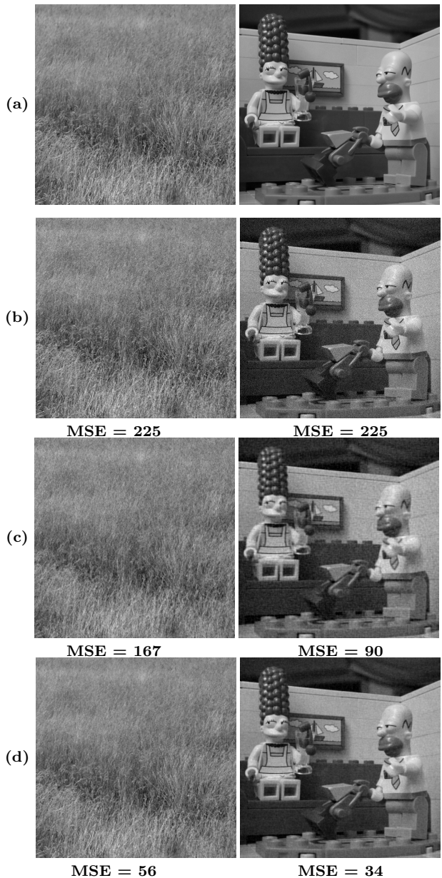
Fig. 1 (a) Original images \mathbf{u} , (b) Noisy images \tilde{\mathbf{u}} with \sigma = 15 , (c) Images \tilde{\mathbf{u}} denoised by hard-thresholding in a DCT basis with a threshold T = \sigma\sqrt{2 \ln N} , (d) Images \tilde{\mathbf{u}} denoised by diagonal estimation with the oracle \lambda^* in a DCT basis.
