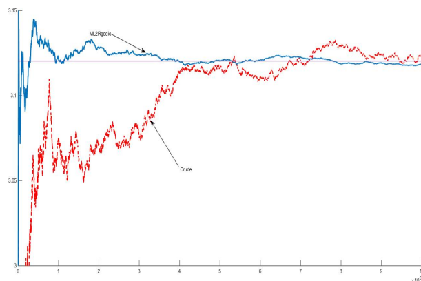
Figure 3: Double-well potential: Approximation of \nu(f) with f(x) = x^2 , \sigma = 2 , Exact value : 3.1207.
