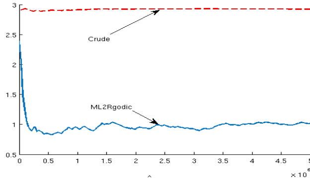
Figure 4: Sparse Regression Learning: n \mapsto \|\hat{\theta}_n - \theta_0\|_2 for the Crude and ML2Rgodic ( R = 3 ) procedures.
