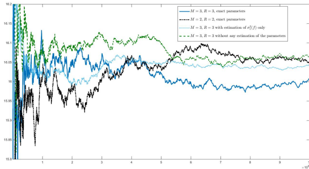
Figure 2: Orstein-Uhlenbeck process: Evolution of the algorithm in terms of the estimation of the parameters, Exact Value : \nu(f) = 16 .
