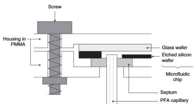
Fig. 4. Scheme of a microfluidic connection.
