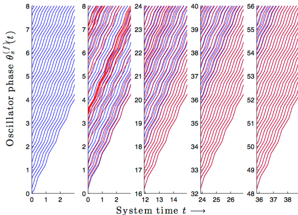
Figure 3: Left panel: Traveling wave solution \theta_s^{(f)}(t) = f(t + \alpha s) for \alpha = 0.2 and s = 1, \dots, 30 vs. time t , together with the forcing signal f (which satisfies condition (C) in Thm 2.1, so as to ensure that the wave is stable – see text). Subsequent panels: Example of a trajectory \theta_s^{(f)}(t) for s = 1, \dots, 30 and disjoint consecutive time windows. The initial phases have been chosen randomly and the forcing signal f is the same as in the left panel. Clearly, the convergence \theta_s^{(f)}(t) \rightarrow f(t + \alpha s) occurs at the first site s=1 and then propagates down the chain, as described in the text; the higher the value of s is, the longer the transient time \theta_s^{(f)}(t) needs in order to get close to f(t + \alpha s) .
