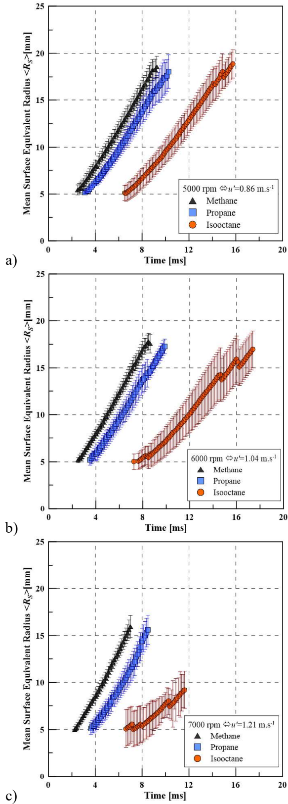
Figure 3. Mean flame radius evolution for the three mixtures: a) 5000, b) 6000 and c) 7000 rpm.
