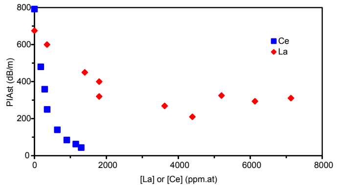
Figure 4: Steady state PIA (PIAst) versus cerium concentration in the Ce (Ce-Al-Tm) series (Blue) and versus lanthanum concentration in the La (La-Al-Tm) series (Red), recorded at 550 nm. Pump power: 1 W. Squares: experimental data.
