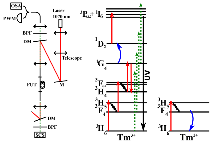
Figure 1: (Left): Experimental setup for PIA measurement. M: dielectric mirror, FUT: fiber under test, BPF: band pass filter, DM: dichroic mirror, OSA: optical spectrum analyzer, SCS: supercontinuum source, PWM: power meter. (Right): Energy level diagram of \text{Tm}^{3+} : red: pump induced transitions, blue: energy transfer, green: 550\text{ nm} probe.
