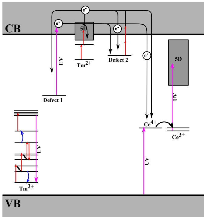
Figure 5: Schematic representation of photo-darkening process, for Tm pumped at 1.07 \mu m . An animated sequence of these mechanisms is available as supplementary material (see Visualization 1).
