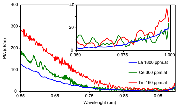
Figure 2: PIA spectra from selected samples after 1.07\text{ }\mu\text{m} laser exposure for 30\text{ min} (pump power 750\text{ mW} ). The resolution is 10\text{ nm} for the \text{La} samples and 1\text{ nm} for the \text{Ce} and \text{Tm} samples. Acquisition time is 10 seconds. Inset: Zoom on the near infra-red region.
