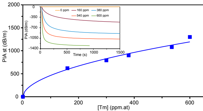
Figure 3: Steady state PIA (PIAst) versus thulium concentration in the Al-Tm-codoped Tm series, recorded at 550 nm. Pump power: 1 W. Squares: experimental data, solid line: power-law fit with exponent = \frac{1}{2} . Inset: corresponding temporal curves.
