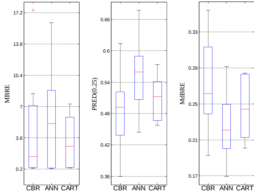
Fig. 2 Boxplots of error metric values of ISBSG dataset
