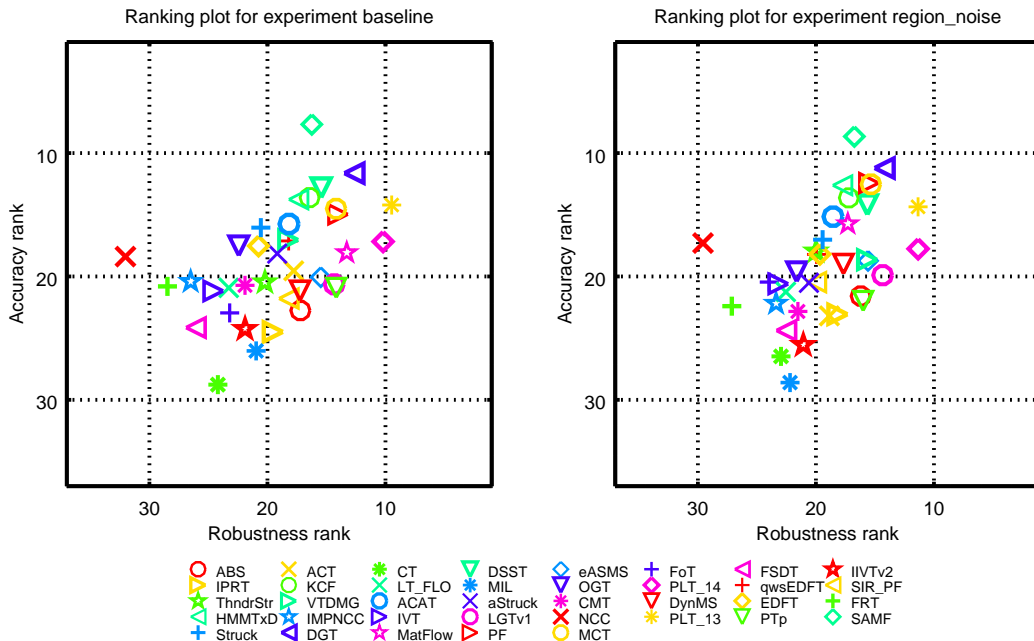
Fig. 2. Accuracy-robustness ranking plots for 39 state-of-the-art methods evaluated with the VOT2014 dataset [43]. The more on the top right, the better. The proposed method MCT (yellow circle) is among the top-performing methods.
