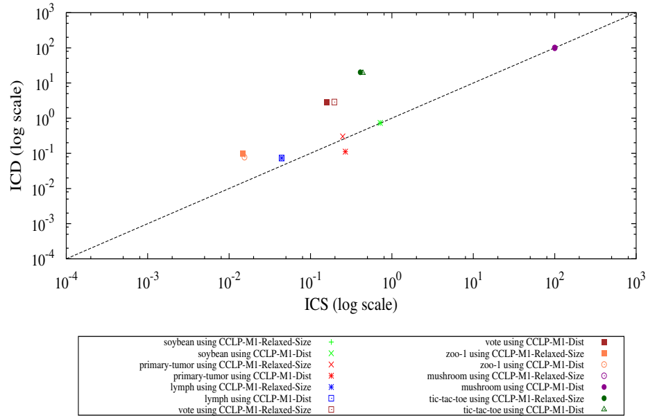
(b) CCLP-M1-relaxed with Size vs. CCLP-M1-Dist.
