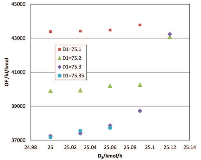
Fig. 5 – Effects of D_1 and D_2 on OF with D_1 , D_2 , F_E , R_1 and R_2 as variables.
