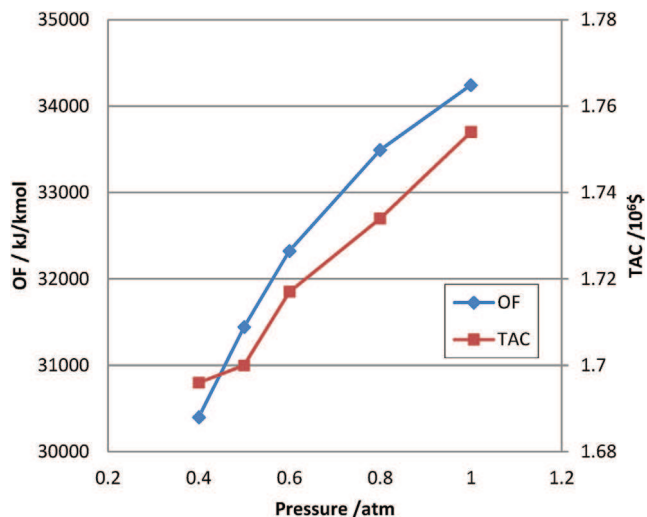
Fig. 9 – Effect of pressure on energy cost OF and TAC.
