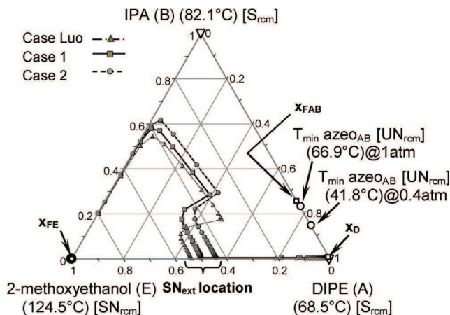
Fig. 8 – Liquid composition profiles for case Luo, cases 1 and 2 extractive distillation column designs for the extractive distillation of DIPE-IPA with 2-methoxyethanol.
