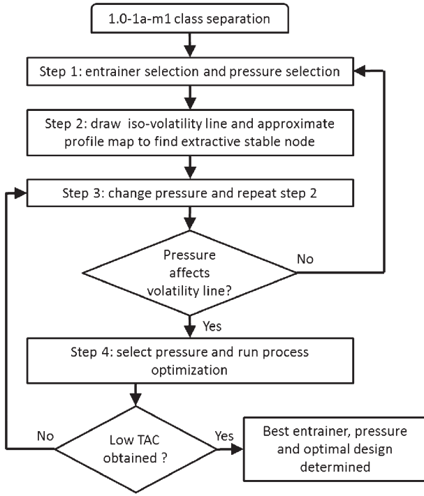
Fig. 2 – Block flow diagram of the proposed methodology for 1.0-1a-m1 extractive separation class.
