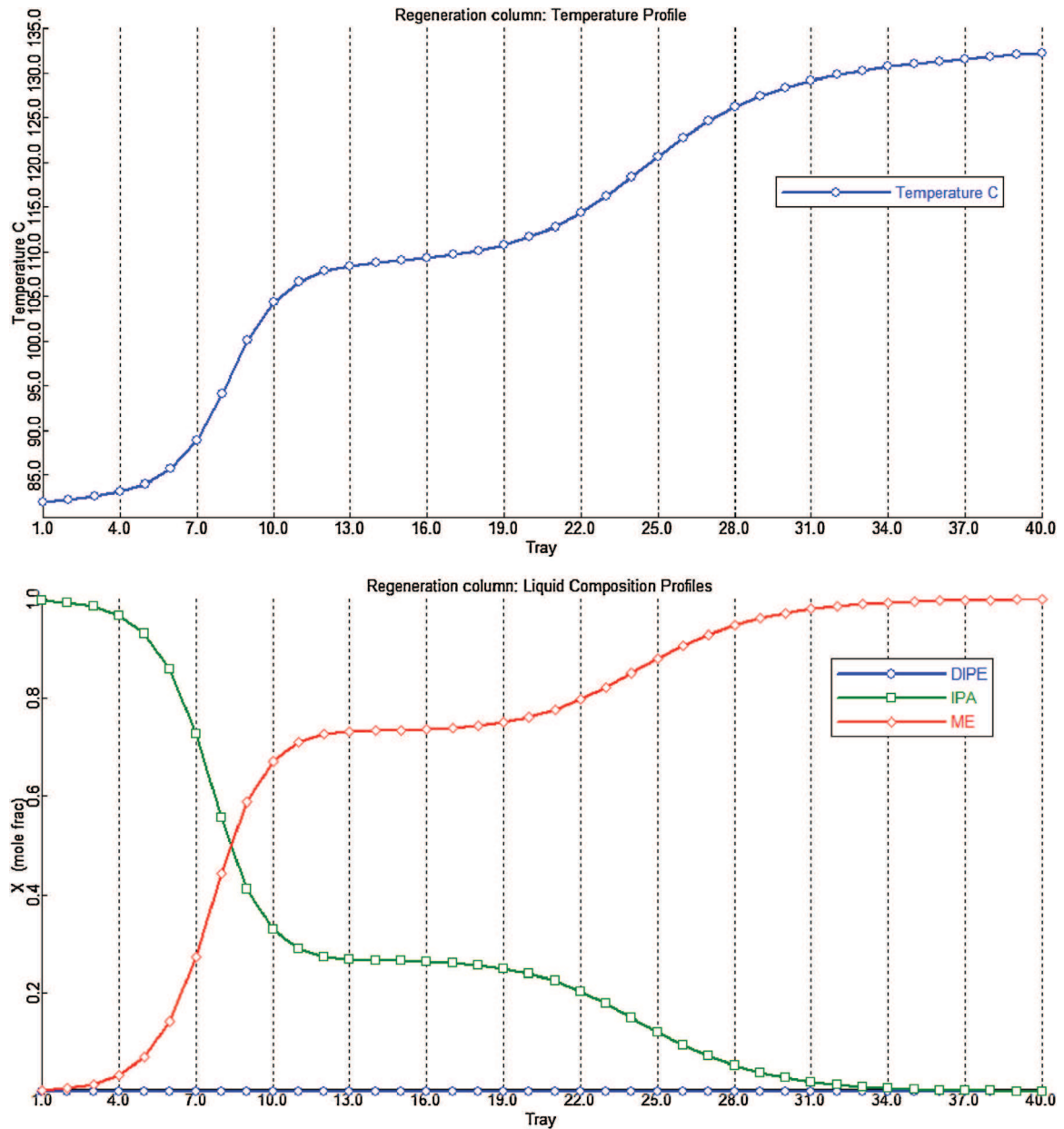
Fig. 7 – Temperature and composition profiles of case 2 entrainer regeneration column for the extractive distillation of DIPE–IPA with 2-methoxyethanol.
