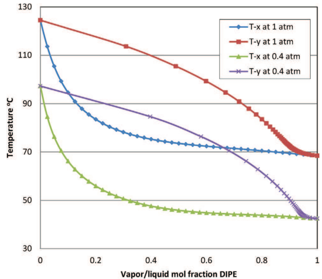
Fig. 4 – T-xy map of 2-methoxyethanol–DIPE.
