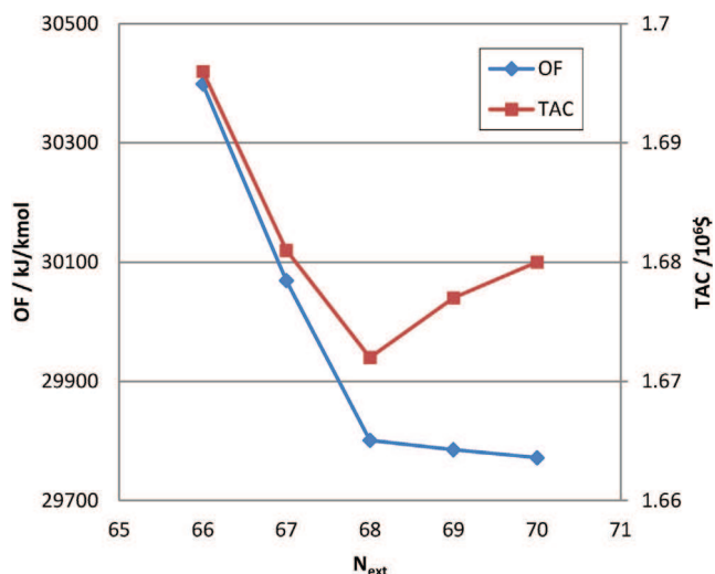
Fig. 10 – Effect of total tray number of extractive column on energy cost OF and TAC.
