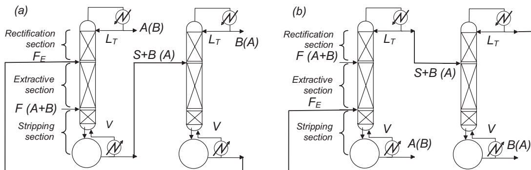
Fig. 1 – Flowsheet of typical extractive distillation with (a) heavy entrainer and (b) light entrainer.
