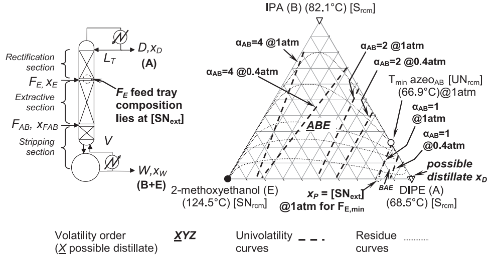
Fig. 3 – Extractive distillation column configuration and DIPE–IPA–2-methoxyethanol. Class 1.0-1a residue curve map at 1atm with isovolatility curves at 0.4 and 1 atm.
