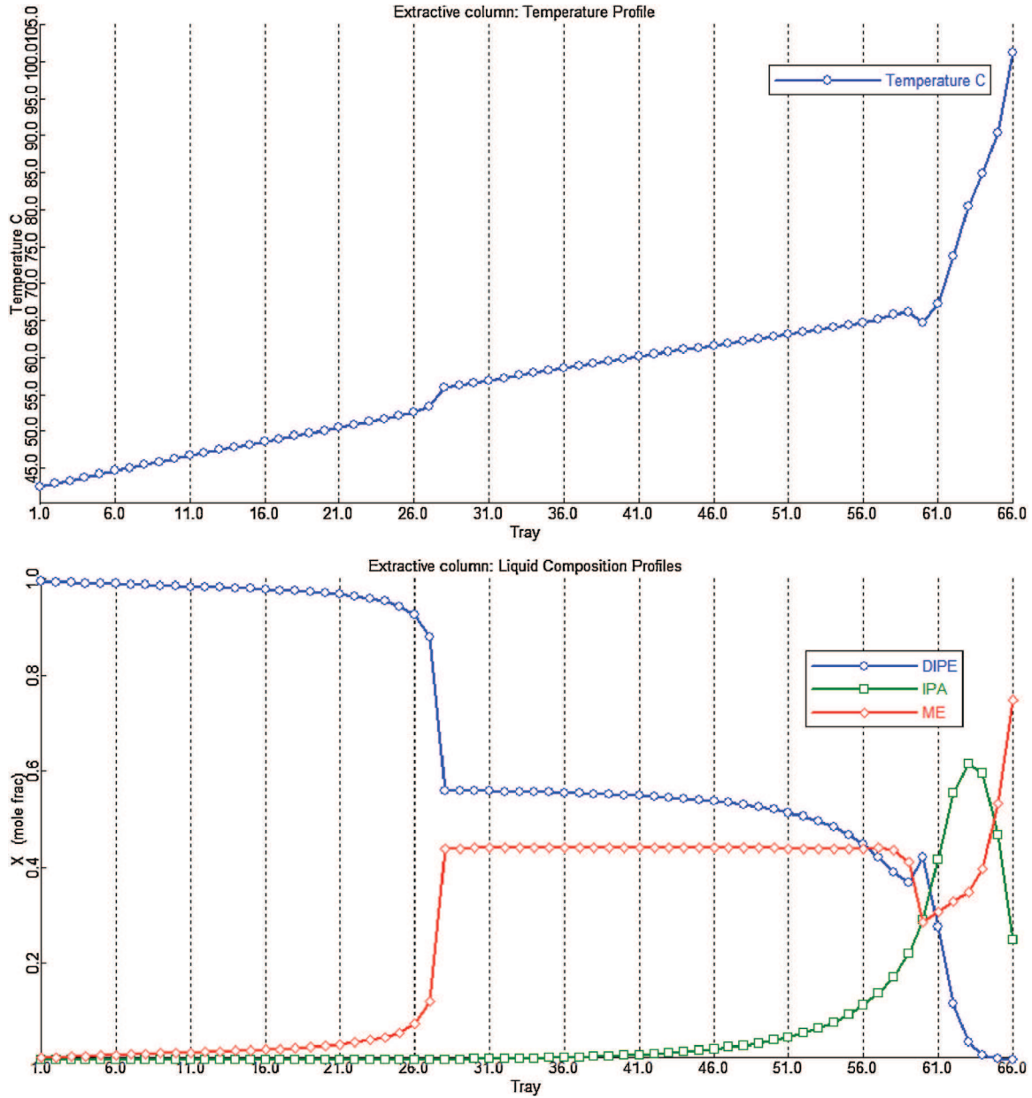
Fig. 6 – Temperature and composition profiles of case 2 extractive column for the extractive distillation of DIPE-IPA with 2-methoxyethanol.
