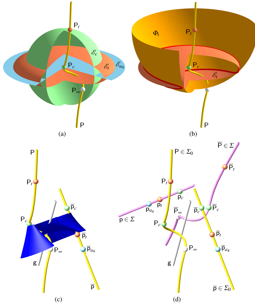
Fig. 1 Type 1 pentapod with self-motion given by a_4 = 2 , A = -1 , C = -5 , a_r = 7 and a_c = 4 . (a) The loci \mathcal{E}_{a_4} , \mathcal{E}_c and \mathcal{E}_t with t = \frac{69}{20} are sliced (along the not drawn axis of rotation c ) in order to visualize their positioning with respect to the cubic P on which the points P_\infty = \sigma(U) , P_c = C and P_t are highlighted. Note that P_{a_4} = W is the real ideal point of P . (b) By setting p_5 = 6 a one-parametric self-motion \mu is fixed. The trajectory of p_t under \mu is illustrated as the intersection curve of \mathcal{E}_t and the sphere \Phi_t centered in P_t . (c) A strip of the basic surface of \mu is illustrated for h_0 = 1 , h_1 = -\frac{489262}{226525} + \frac{488}{226525}\sqrt{675091} and h_2 = \frac{535336}{226525} + \frac{446}{226525}\sqrt{675091} . In addition P and \bar{p} are visualized, where the latter denotes the pose of \bar{p} such that its half-turns about the generators of the basic surface yield the self-motion \mu . (d) Kramers's construction is illustrated with respect to the generator g of the basic surface: As P_{a_4} (resp. \bar{p}_\infty ) is the real ideal point of P (resp. \bar{p} ), the trajectory of p_{a_4} (resp. \bar{P}_\infty ) under \mu is planar. The (Mannheim) plane \Sigma , which contains the point P_\infty (resp. \bar{p}_{a_4} ) and is orthogonal to the direction of the real ideal point p_\infty (resp. \bar{P}_{a_4} ) of p (resp. \bar{P} ) in the displayed pose, slides through the point P_\infty (resp. \bar{p}_{a_4} ) during the complete motion \mu .
