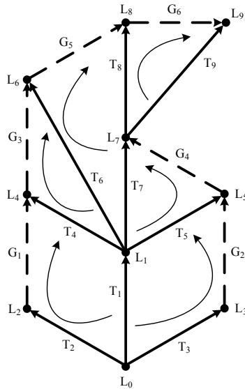
Fig. 3 Associated digraph
