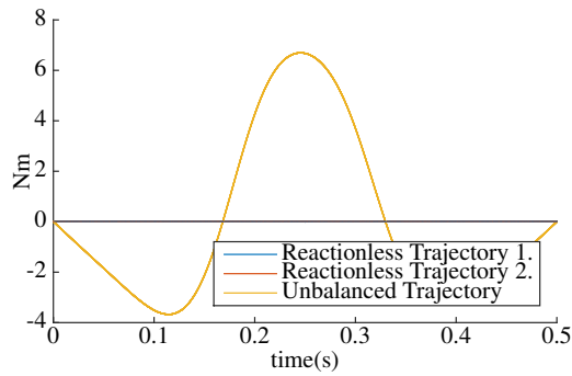
Fig. 4: Shaking moments
