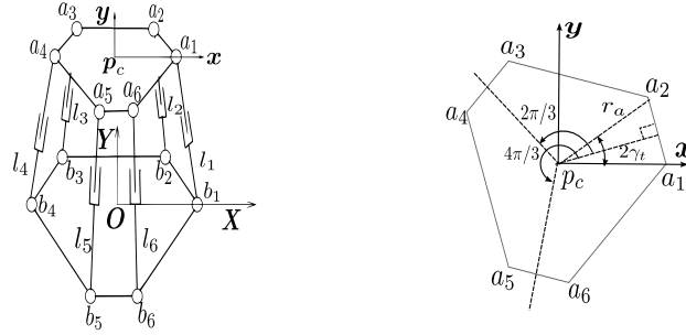
(a) Schematic diagram of SRSPM. (b) Geometry of the top platform.
