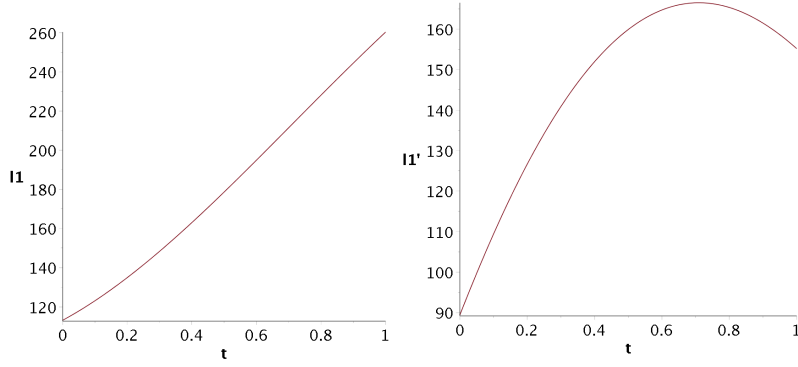
Fig. 3 First time derivative of the explicit joint function of leg l_1
