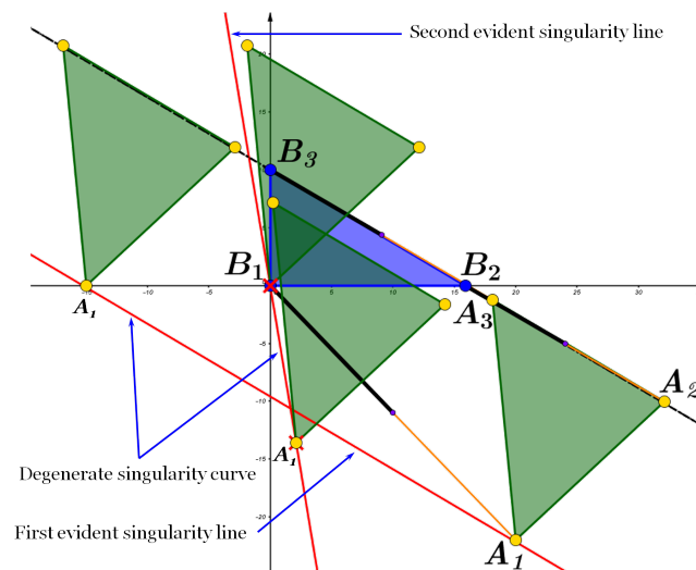
Fig. 3 Degenerate singularity curve of the 3\text{-RRR} manipulator
