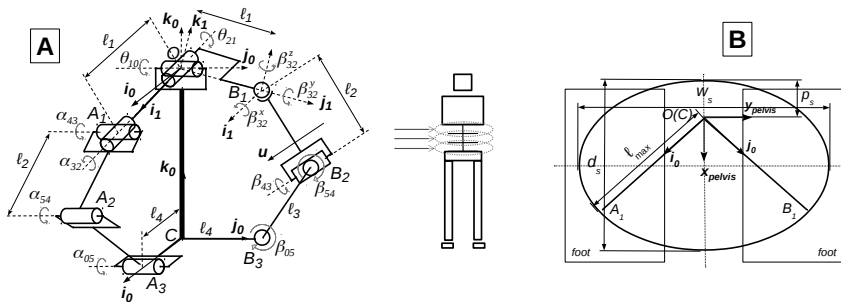
Fig. 1 A. Perspective view of one parallel mechanism module after pitch and roll rotations, resp. about fixed axis j_0 , and about axis i_1 . B. Top view of waist and footprints. Available volume : height h_s = 0.30[m] , width, w_s = 0.25[m] and depth d_s = 0.20[m] .
