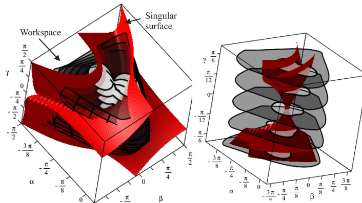
Fig. 4 Workspace, singular surface, and workspace slices and singularities.
