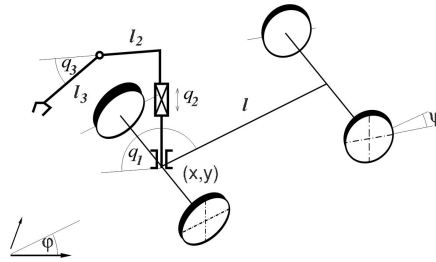
Fig. 1 Mobile manipulator
