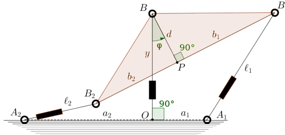
Fig. 3 The modified manipulator
