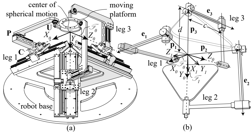
Fig. 2 Virtual model (a) of the spherical 3-CPU manipulator Sphe.I.Ro. Reference frames and geometrical parameters of the i^{\text{th}} leg (b).
