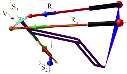
Fig. 3 A singular configuration of the surgical robot.
