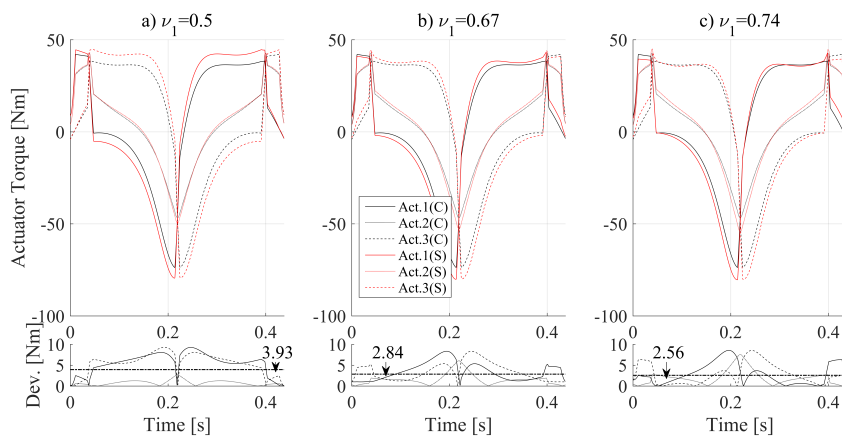
Fig. 4 Comparison of the deviations of actuator torques
