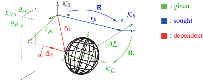
Figure 2 Definition of the pressure point for a generic ellipsoid.
