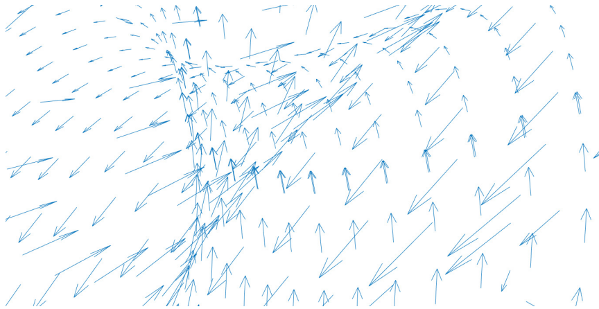
Fig. 9 A Linear Velocity Field: \dot{\theta}_s = 0 .
