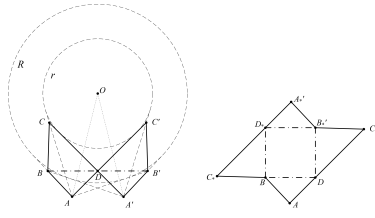
Fig. 4 Example of the type III Bricard linkage
