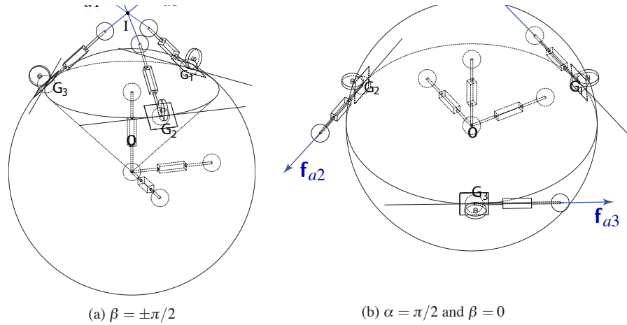
Fig. 5: Singular configurations of the parallel spherical wrist
