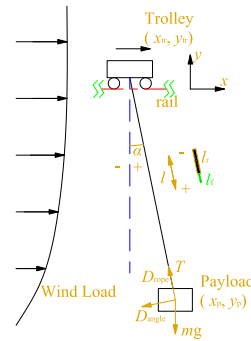
Fig. 2 Trolley-payload coordinate system
