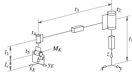
Fig. 3: Basic structure of the 1st PRPR chain
