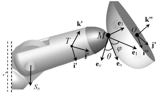
Fig. 2 The Darboux frames (M - \mathbf{e}_u \mathbf{e}_e, \mathbf{e}_3) , (M - \mathbf{e}_\alpha \mathbf{e}_\beta \mathbf{e}_3) , and (M - \mathbf{e}_1 \mathbf{e}_2 \mathbf{e}_3) at the contact point M
