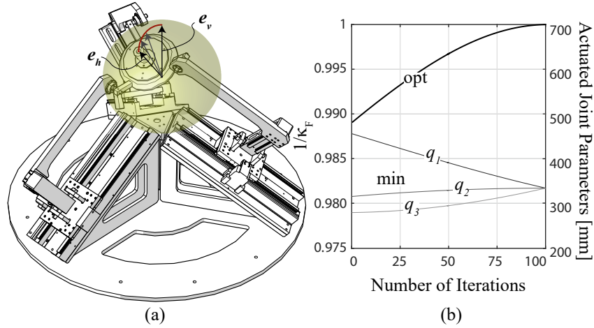
Fig. 3 (a) Sphero-I.Ro PKM in the arbitrary initial posture of the trajectory; (b) reciprocal of the condition number for SQP and function evaluation and joint values progressions.
