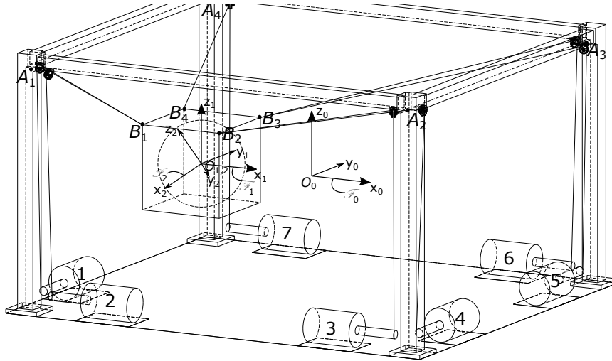
Fig. 2: Concept idea of the manipulator
