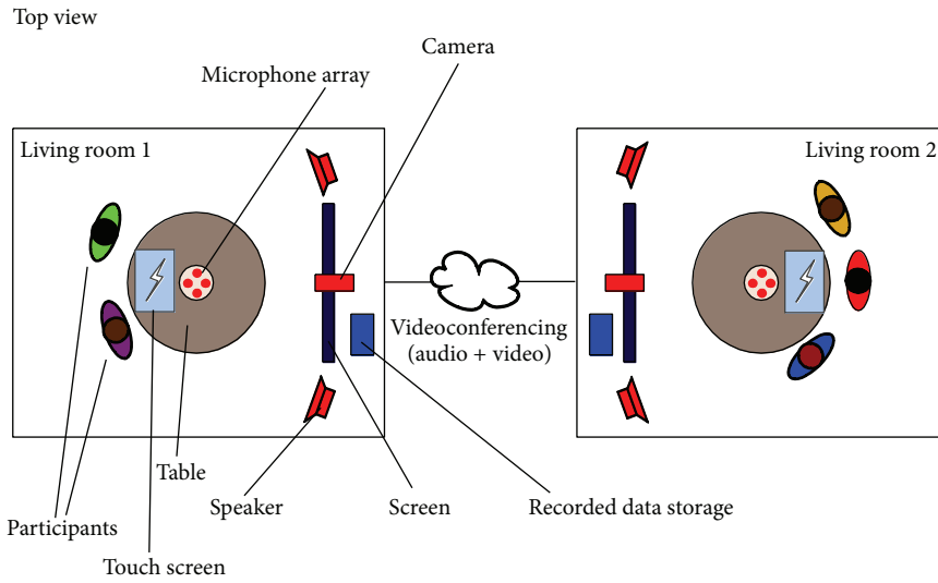
FIGURE 1: TA2 setup, view from top [36]. The audio and video sensors are spatially separated within a room: the microphone array is located above the table next to participants, while the camera is collocated with the wall screen for teleconferencing.
