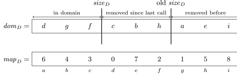
Fig. 4. If “old size_D ” was the size of D on the last propagation of a constraint, the values c , b and h have been removed since then. To perform incremental propagation, the propagator only has to check the values for which c , b or h was a support. Note that the “old size_D ” marker is a property of the propagator and is different for each propagator, while size_D is a property of D .
