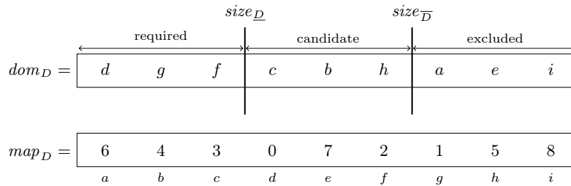
Fig. 6. Example representation of the domain \underline{D} = \{d, g, f\} , \overline{D} = \{d, g, f, c, b, h\} . The size_{\underline{D}} first values belong to \underline{D} ; the size_{\overline{D}} first values belong to \overline{D} . In such representation, only size_{\underline{D}} and size_{\overline{D}} need to be kept in the trail.
