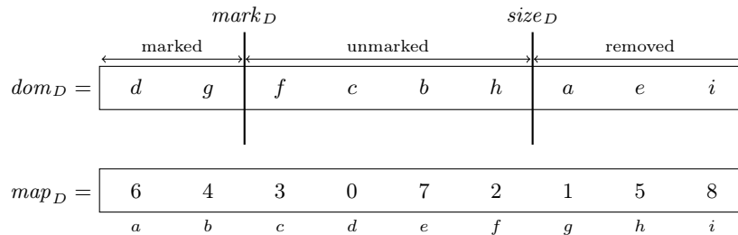
Fig. 3. Values can be marked in the discrete representation of a domain by moving the value to the beginning of the dom_D array and increasing the mark_D marker. To restrict the domain to only the marked values, we only need to set size_D to mark_D .
