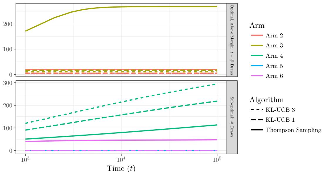
Figure 2: Time minus the number of optimal arm draws (top) and number of suboptimal arm draws (bottom) in Simulation 4.
