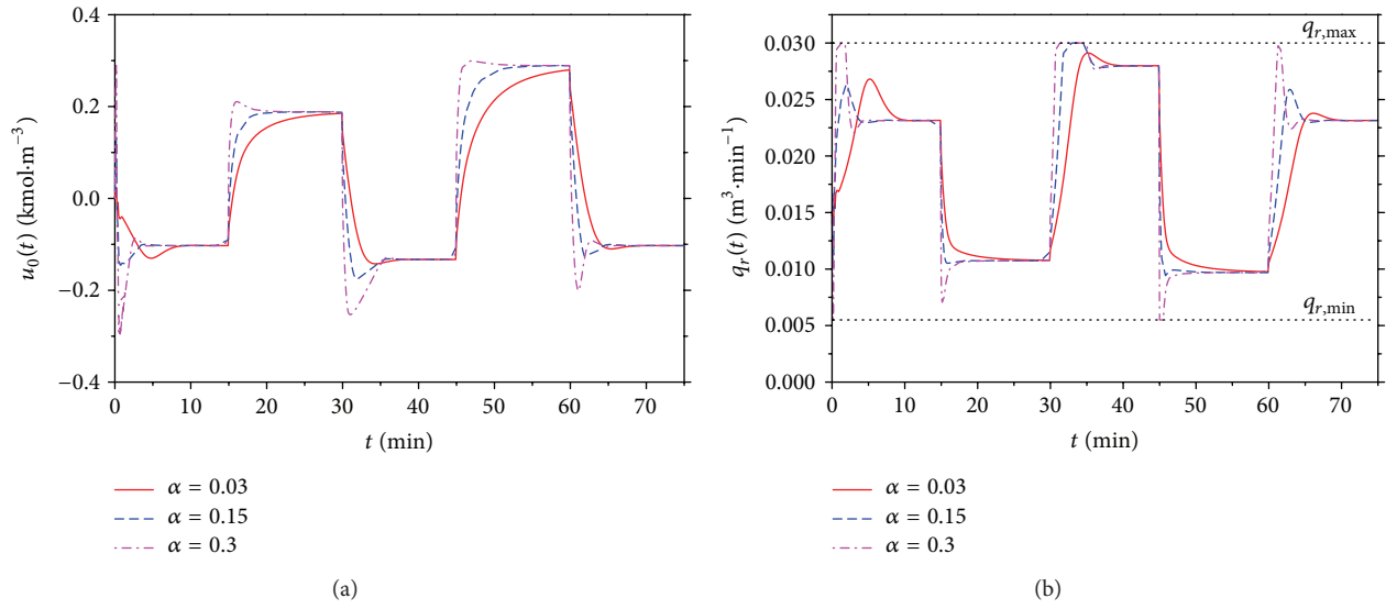
FIGURE 13: Outputs from the LDP u_0 or various values of \alpha (a) and the courses of the computed input variable, q_r , to the ELM for various \alpha (b).
