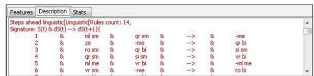
FIGURE 13: Winning predictor linguistic description (trend-cycle model).
