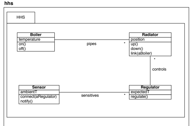
Fig. 2 Model hhs of home heating systems
