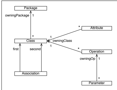
Fig. 1 Class metamodel
