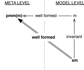
Fig. 30 Sketch of Property 14
