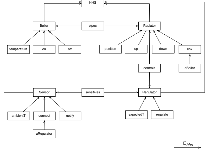
Fig. 3 Representation of hhs (Figure 2) in the formalism
