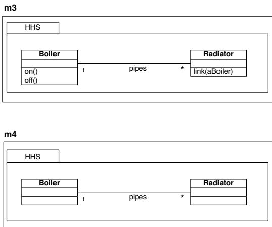
Fig. 5 Transitivity invariant submodels of “home heating systems” model (Fig. 2)
