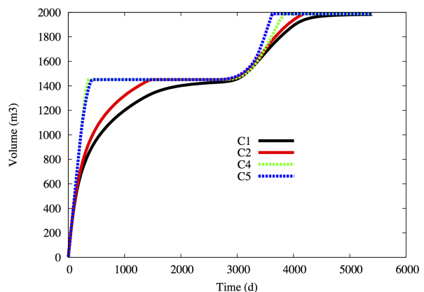
Fig. 20: Amount of oil in the faults in m 3 as a function of time for the following four test cases. C_1 : b_m = 10^6 Pa, b_f = 10^5 Pa, p_{ent,m} = p_{ent,f} = 0 , C_2 : b_m = 10^6 Pa, b_f = 0 , p_{ent,m} = p_{ent,f} = 0 , C_4 : b_m = 10^6 Pa, b_f = 0 , p_{ent,m} = 10^6 Pa, p_{ent,f} = 0 , C_5 : b_m = b_f = 0 , p_{ent,m} = 10^6 Pa, p_{ent,f} = 0 .
