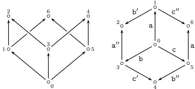
FIGURE 5. Two views of the Hasse diagram of the local lattice P_A that satisfies Condition (6.3), hence such that the associated system \mathcal{R}(\Upsilon(P_A)) is semi-convergent.
