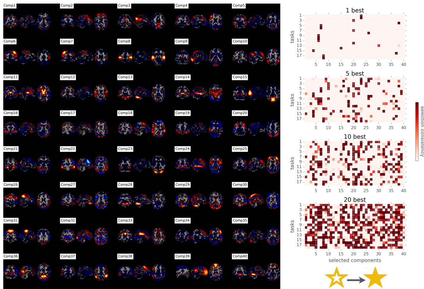
Fig 4. Network co-occurrence modeling: Sparse PCA network decomposition of ARCH1 task maps and network-task assignment. 40 network components underlying 18 ARCH1 tasks have been discovered by sparse PCA (Comp1–40 on the left). The ensuing network loadings from the second half of the ARCH1 task data were submitted to classification of the psychological tasks based on the implication of brain networks (l2-penalized support vector machines, multi-class, one-versus-rest). l2-penalized support vector machines was employed to choose the most discriminative network variables by a preceding classical univariate test in a discrete fashion rather than by sparse variable selection based on l1 penalization (cf. methods section). This diagnostic analysis (right) revealed the most distinctive k = 1, 5, 10 , and 20 network features (red cubes) for each experimental condition of the task battery (cf. Fig 3). The thus discretely selected network features per task were then fed into supervised multi-task classification as a feature space of activity-map-wise continuous activity values. The color intensity of the k cubes quantifies how often the corresponding brain network was selected as important for a task across cross-validation folds. This diagnostic test performed inference on a) the single most discriminative network for each task at k = 1 , b) the network variables that are added step-by-step to the feature space of network implications with increasing k , and c) what network variables are unspecific (i.e., not selected) for a given task at k = 20 . See tables for the corresponding descriptions of task 1–18. See S1–S3 Figs for analogous plots based on different matrix factorizations and datasets.
