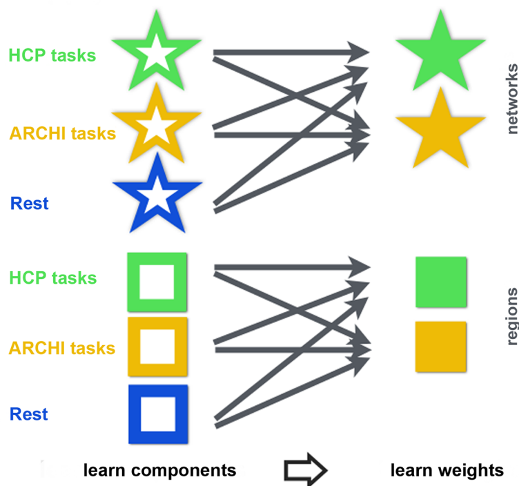
Fig 1. Overview of experimental analyses. The schematic summarizes the modeling experiments undertaken in the present study. Symbols are introduced that describe how the HCP task data (green), the ARCHI task data (yellow), and the rest data (blue) were used to (A) evaluate the idea of network co-occurrence modeling and (B) test explicit hypotheses about the commonalities and differences between human brain activity in task-constrained and idling brain states [3, 6]. Stars indicate brain networks derived as mutually overlapping spatiotemporal patterns from independent component analysis (ICA), principle component analysis (PCA), sparse PCA, and factor analysis (FA). Cubes indicate discrete brain regions derived as mutually disjoint voxel groups from k-means and ward clustering. Empty stars or cubes indicate learning a network decomposition or region segregation from brain activity maps without the task labels (i.e., "unsupervised statistical learning"). Filled stars or cubes indicate learning a classification algorithm of 18 typical psychological tasks based on brain activity maps summarized as networks or regions with the task labels (i.e., "supervised statistical learning"). The origin of the arrows indicate from what data (HCP tasks, ARCHI tasks, or rest) the networks and regions were obtained. The arrows point to the set of psychological
