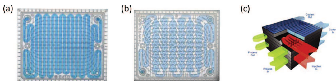
Fig. 1. Millistructured reactors: (a) Corning RT, (b) Corning HP and (c) Chart ShimTec ® [9,10].
