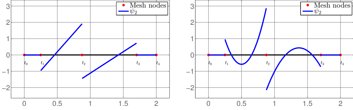
FIGURE 1. The basis function \psi_2 from (4) for polynomial degrees p = 1 (left) / p = 2 (right).
