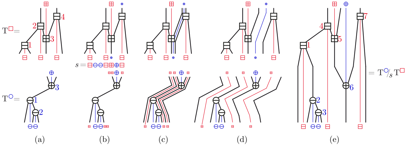
Fig. 7: (a) Two Cambrian trees T^{\circ} and T^{\square} . (b) Given the shuffle s = \square \circ \square \square \square \oplus \oplus \oplus of their signatures, the positions of the \square are reported in T^{\circ} and the positions of the \oplus are reported in T^{\square} . (c) The corresponding laminations. (d) The trees are splitted according to the laminations. (e) The resulting Cambrian tree T^{\circ}/_s T^{\square} .
