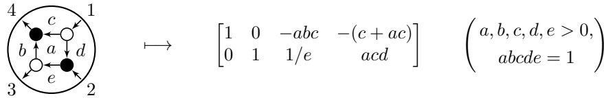
Fig. 1: A homeomorphism from \mathbb{R}_{>0}^4 to the cell of \text{Gr}_{2,4}^{\geq 0} labeled by the positroid M = \binom{[4]}{2} .
