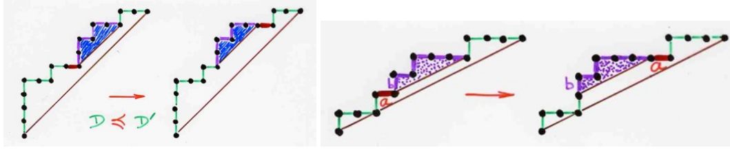
Fig. 3: The Tamari covering relation for ballot (Dyck) path (left). The covering relation in the m -Tamari lattice ( m=2 ) (right).
