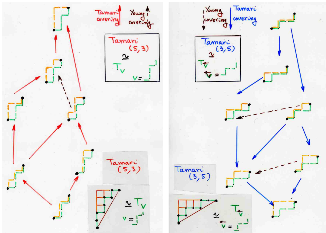
Fig. 5: Duality and rational Catalan combinatorics: the lattices \text{Tam}(5,3) and \text{Tam}(3,5) .
