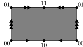
Fig. 4: (\mathbb{R}^2 - \mathbb{Z}^2)/G
