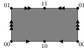
Fig. 4: (\mathbb{R}^2 - \mathbb{Z}^2)/G
