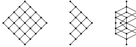
Fig. 1: Some doubled root posets
