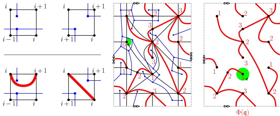
Fig. 4: Left-Top: face-types after the construction of \nabla(q) . Left-Bottom: constructing \Phi(q) from \nabla(q) . Middle and Right: Construction (in red) of the labeled unicellular map \Phi(q) associated to the bipartite quadrangulation from Fig. 3.
