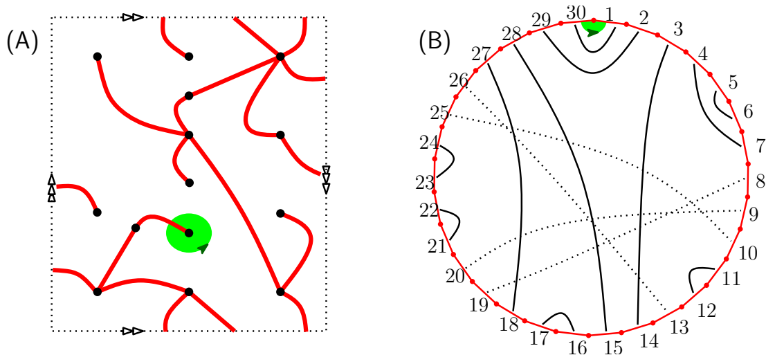
Fig. 1: (A) A unicellular map drawn on a Klein bottle \mathcal{N}_1 (opposite sides of the dotted rectangle should be glued together as indicated by arrows); (B) The same map represented as a polygon with glued sides (straight and twisted gluings are indicated by plain and dotted lines, respectively). The corresponding sets of matchings are E_s(\mathcal{M}) = \{\{1, 30\}, \{2, 29\}, \{3, 14\}, \{18, 27\}, \{23, 24\}, \{22, 21\}, \{16, 17\}, \{11, 12\}\} , and E_t(\mathcal{M}) = \{\{13, 26\}, \{10, 25\}, \{9, 20\}, \{8, 19\}\} .
