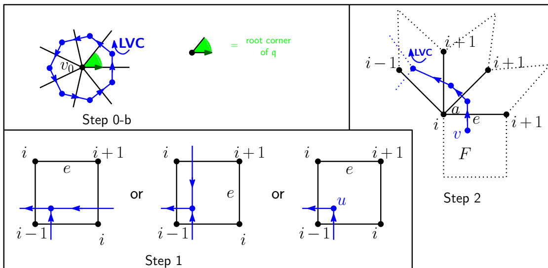
Fig. 2: The construction of \nabla(q) . Top: Step 0b; Bottom: the face F and the edge e selected by Step 1; Right: Step 2.
