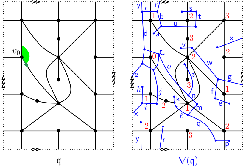
Fig. 3: Left: A rooted quadrangulation q on the Klein bottle \mathcal{N}_1 . Right: The associated dual exploration graph \nabla(q) is depicted in blue. To help the reader visualize the construction, we have numbered the blue edges appearing after Step 0 by a, b, \dots, z in their order of appearance in the construction. We have not indicated the orientation of these edges, to make the picture lighter.
