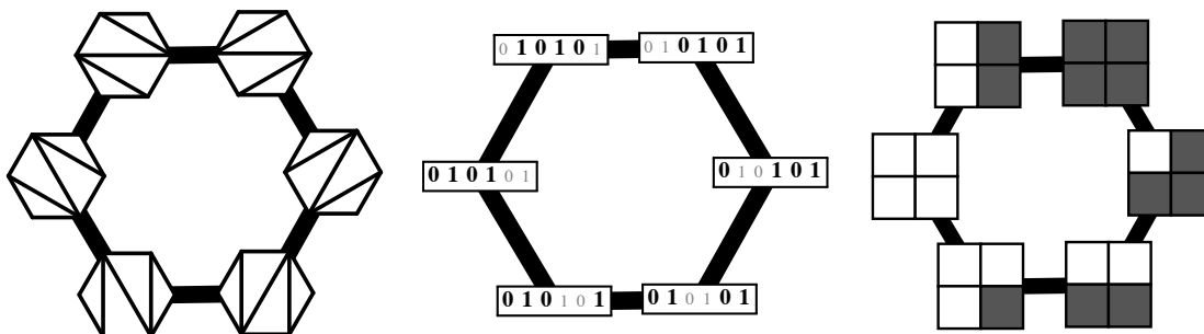
Fig. 4: From left to right, we have \text{Tri}_B(6, 1) , \mathcal{S}(B_2, 1) , and \mathcal{J}(A_{2n-1}^n, 1) . The graph structure is given by flips.
