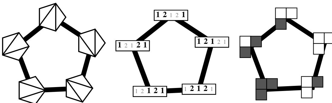
Fig. 3: From left to right, we have \text{Tri}_A(5, 1) , \mathcal{S}(A_2, 1) , and \mathcal{J}(A_n, 1) . The graph structure is given by flips. With the proper orientation, the graph at the left recovers the Tamari lattice on Dyck paths.
