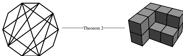
Fig. 1: An example of the bijection in Theorem 2 for n = 3 and k = 2 . On the left is a 2-triangulation of a 10-gon; on the right is the corresponding plane partition of height 2 in a square of size 3.
