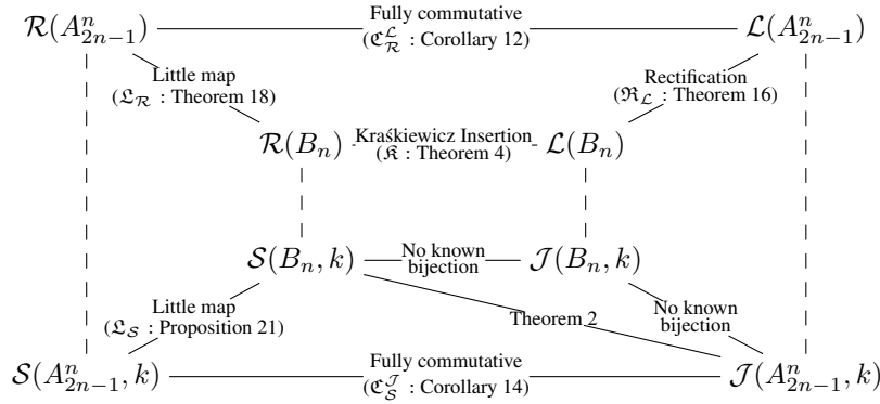
Fig. 2: The bijections between \mathcal{R}, \mathcal{L}, \mathcal{S} , and \mathcal{J} for B_n and A_{2n-1}^n .
