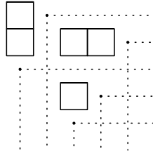
Figure 1: Rothe diagram of w = [25143] (corresponding to the positions of the black dots above) is D(w) = \{(1, 1), (2, 1), (2, 3), (2, 4), (4, 3)\} (shown by the boxes above).
