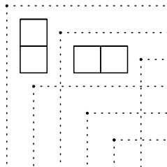
Figure 2: Rothe diagram of a Grassmannian permutation w = [136245] . Here u_w = (u_2 \wedge u_3) \otimes u_3 \otimes u_3 is a lowest vector in an irreducible representation of \mathfrak{gl}_3 with lowest weight (0, 1, 3) .
