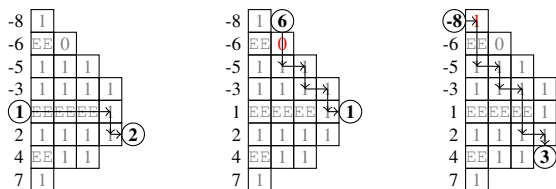
Fig. 3: Zigzag maps in permutation tableaux of type B .
