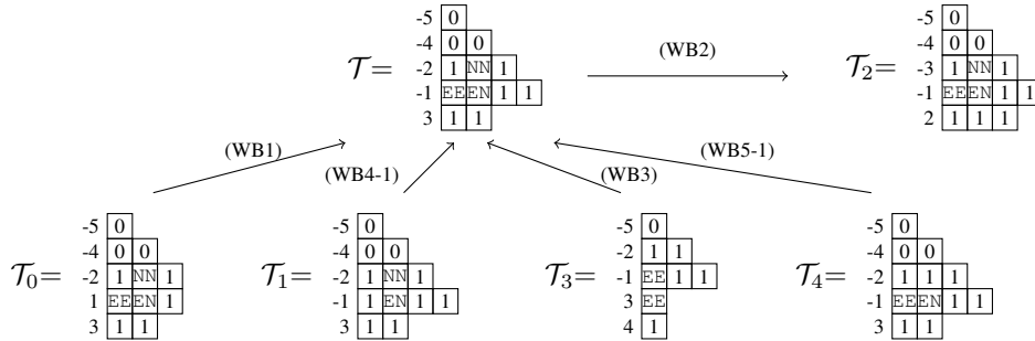
Fig. 11: All covering relations in weak Bruhat order including T .
