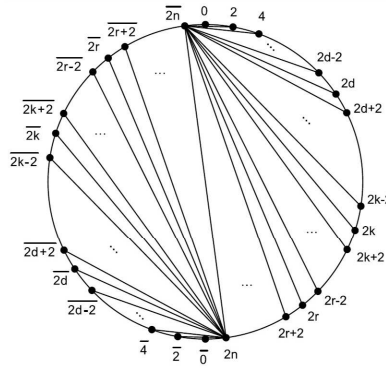
Figure 1: The initial cluster of \mathcal{A}_n
