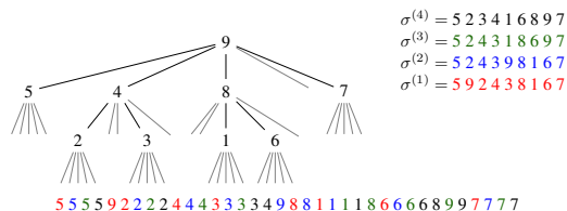
Figure 4: A 5-decreasing tree, its corresponding metasylvester 4-chain and maximal class element
