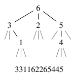
Figure 2: An element of \mathcal{DT}_6^{(3)} and its corresponding element of \text{Max}_6^{(2)} .
