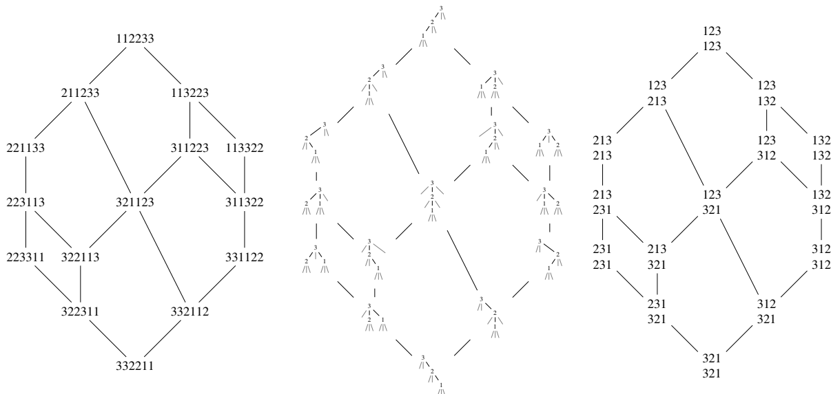
Figure 3: The metasylvester lattice on \text{Max}_3^{(2)} , \text{DT}_3^{(3)} , and \text{MC}_3^{(2)} . (in the third lattice \sigma^{(2)} is at the top of each list and \sigma^{(1)} at the bottom).
