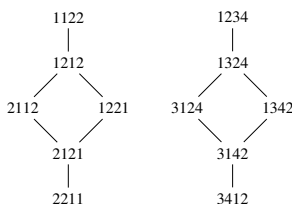
Figure 1: Lattice on \mathfrak{S}_2^{(2)} as an ideal of the right weak lattice on \mathfrak{S}_4 .
