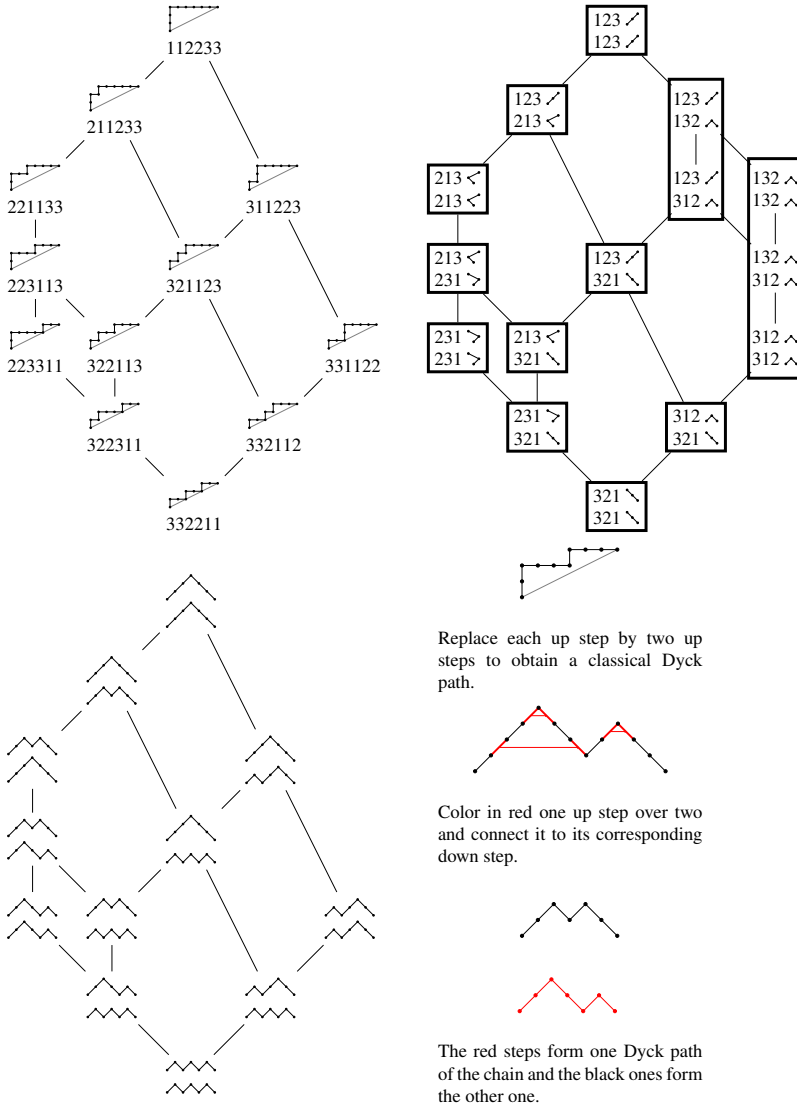
Figure 6: On the top: the m -Tamari lattice as a sublattice and quotient lattice of the metasylvester lattice. On the bottom: the realization of m -Tamari in terms of chains of Dyck paths.
