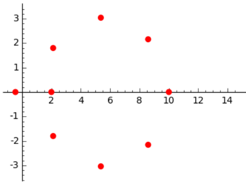
Fig. 1: Roots of p_{\{2,10\}}(z) .
