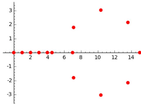
Fig. 2: Roots of p_{\{4,7,15\}}(z) .
