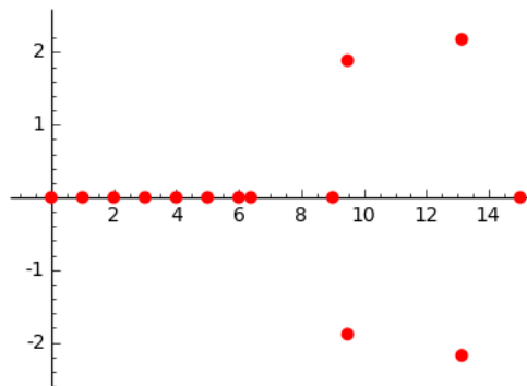
Fig. 4: Roots of p_{\{4,6,9,15\}}(z) .
