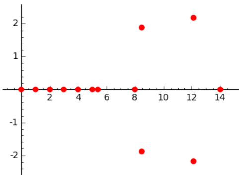
Fig. 3: Roots of p_{\{3,5,8,14\}}(z) .
